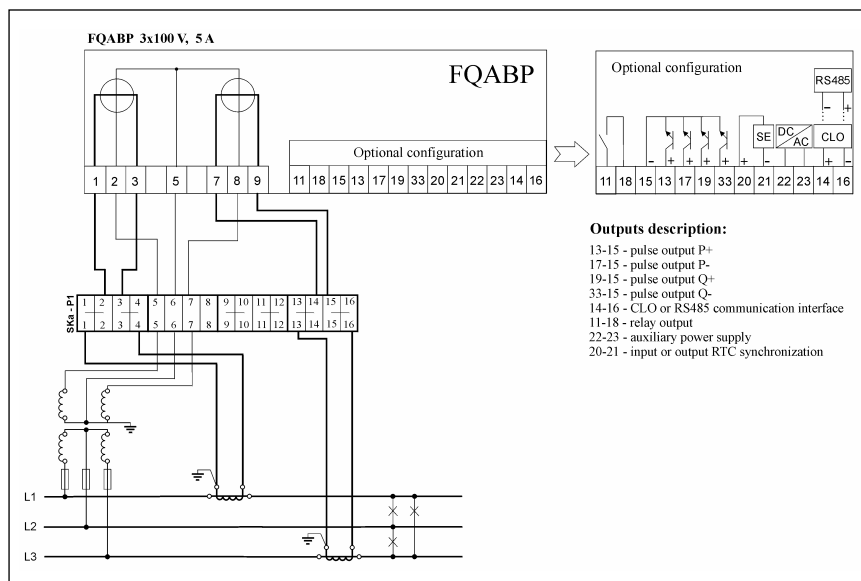
Exemplary connection diagram
